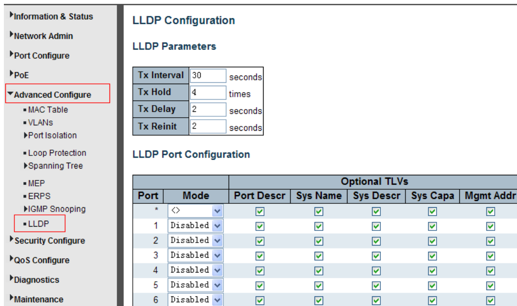
Figure 5-9 LLDP Configuration Screen
