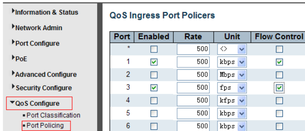
Figure 6-2Port PolicingConfiguration Screen
