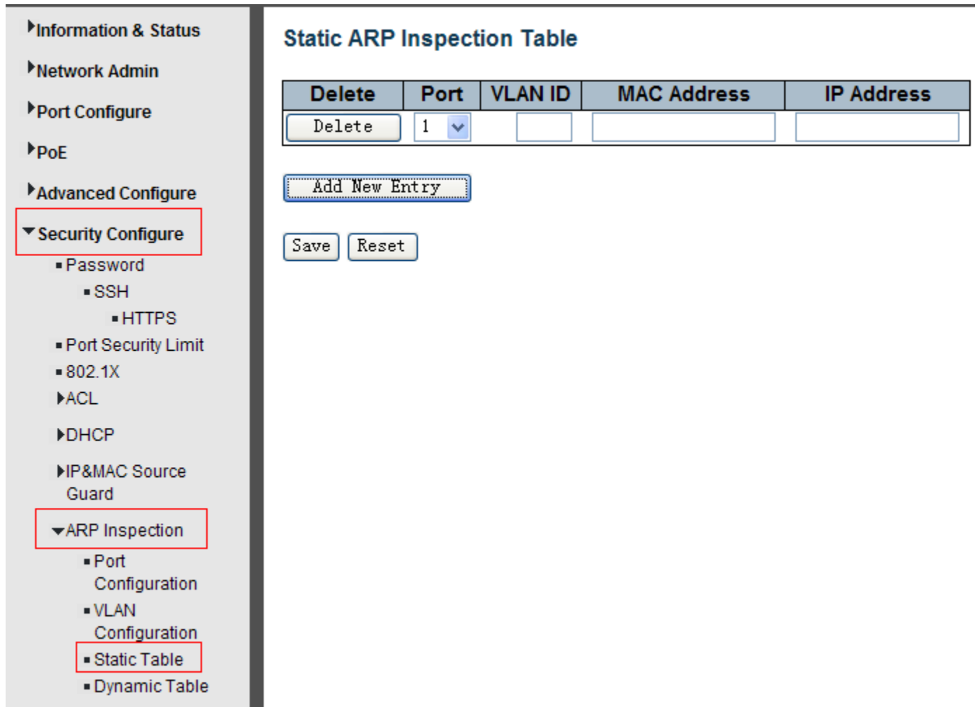
Figure 7-9 Static Table Configuration Screen
