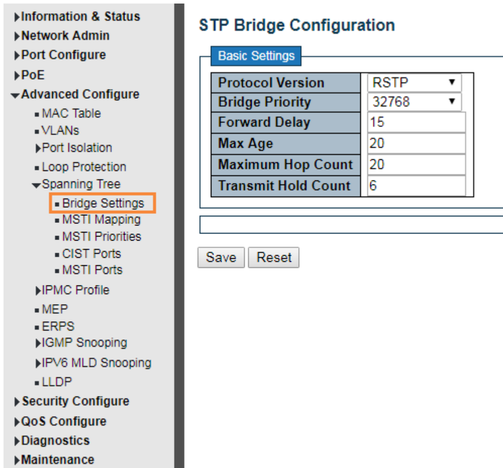
Figure 5-4 Spanning Tree Configuration Screen
